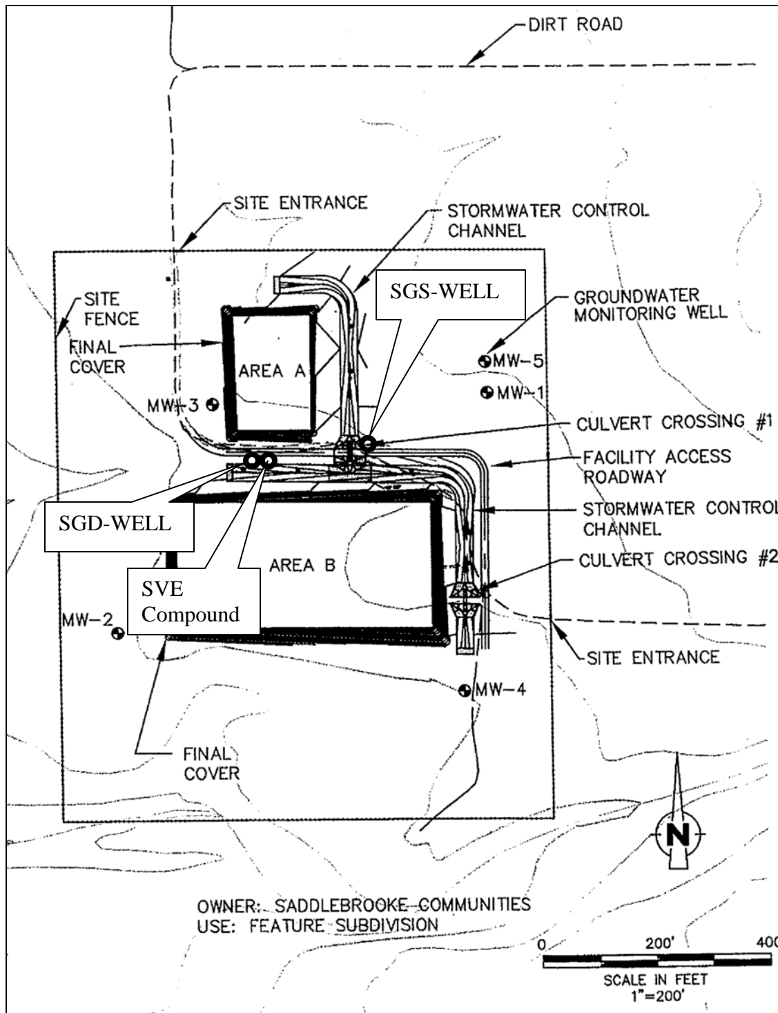
Figure 2. University of Arizona Page Trowbridge Ranch Landfill ground water and vapor monitoring system near Oracle Junction and the Town of Oracle, Arizona.
