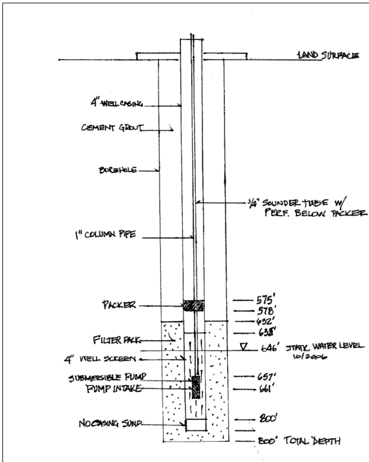
Figure 4. PTRL ground water monitoring well MW-2 construction drawing showing the inflatable packer installed so that the well may also be used as a soil vapor monitoring point.
