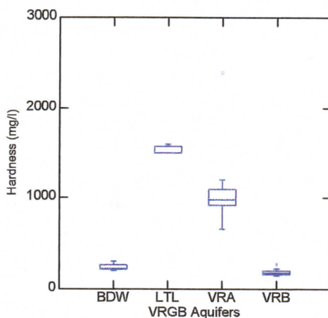
Figure 5. Boxplot comparing hardness levels among four VRGB aquifers.
