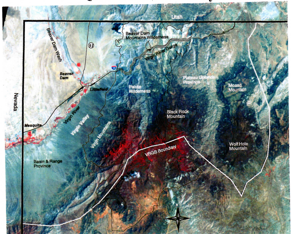
Figure 2. In this infra-red satellite image of the Virgin River basin (outlined in white), riparian vegetation, irrigated farmland, and, near mountain summits, juniper forest appear in crimson.
