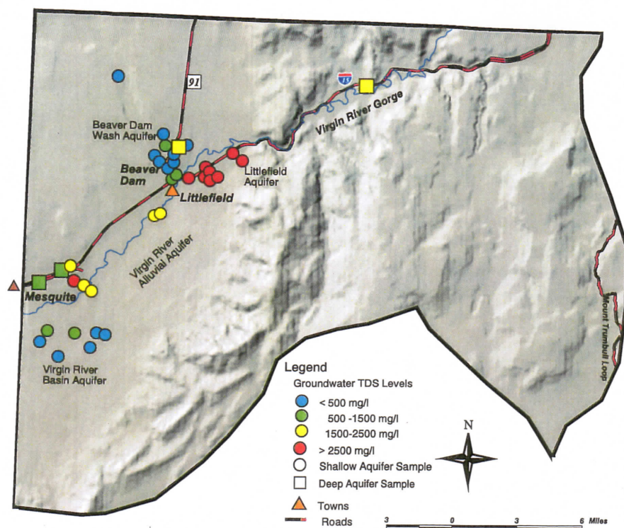
Figure 4. Total dissolved solids (TDS) concentrations are shown at 38 sampling sites. High TDS is the main limitation in using groundwater for domestic use in the VRGB.
