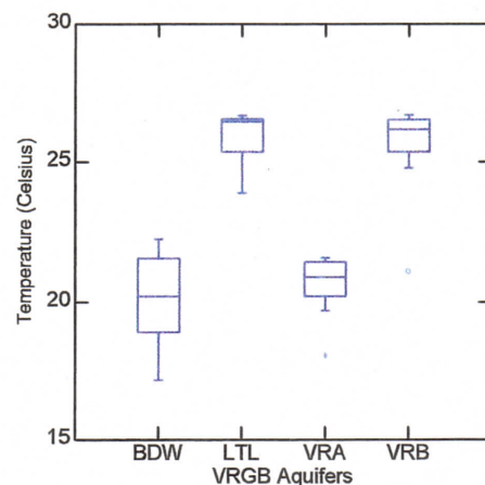
Figure 7. Boxplot comparing temperature levels among four VRGB aquifers.
