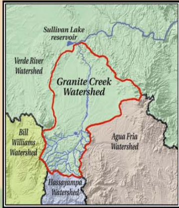
Granite Creek Watershed & Adjacent Watersheds
