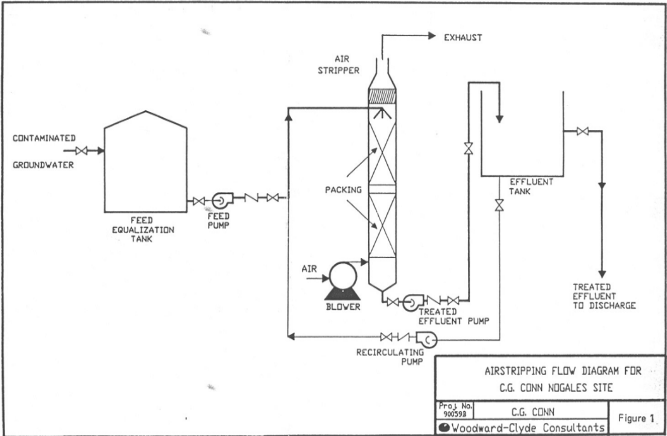
Figure 3 - Schematic of Conn-Selmer's Groundwater Remediation System (GRS)
