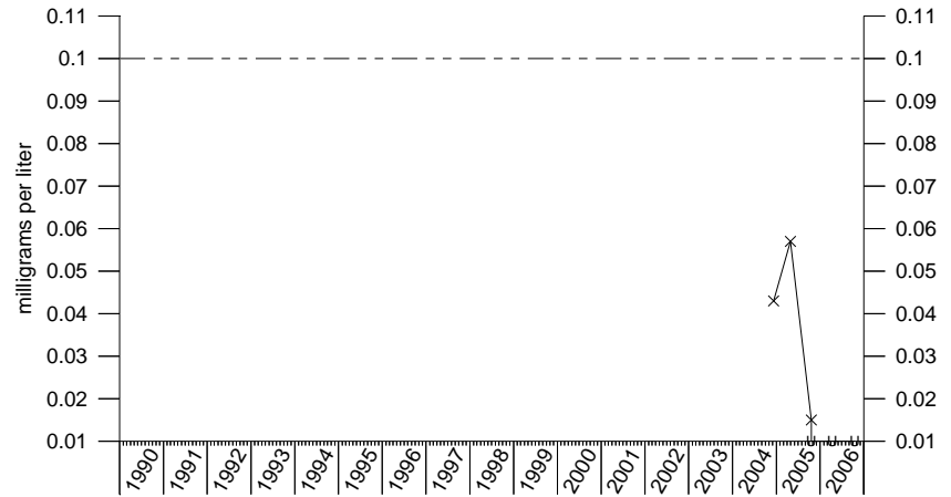
Chromium IRA-29
