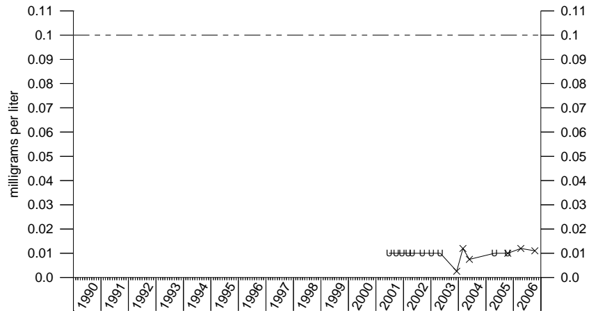
Chromium IRA-12-210
