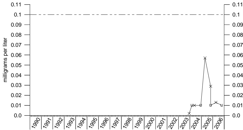
Chromium IRA-21
