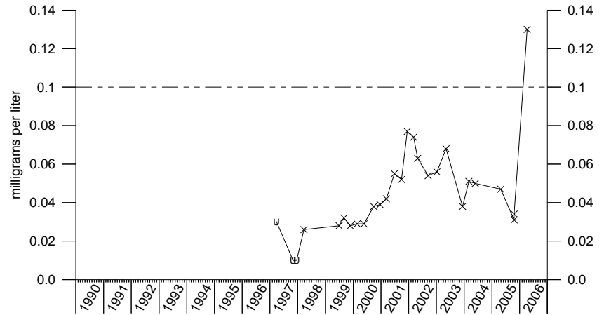
Chromium IRA-8
