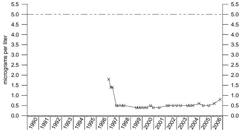
Tetrachloroethene IRA-12-210
