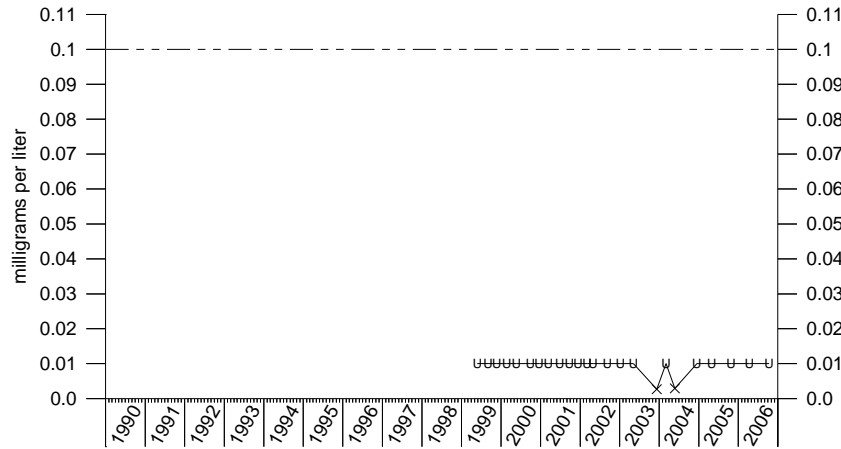
Chromium IRA-1
