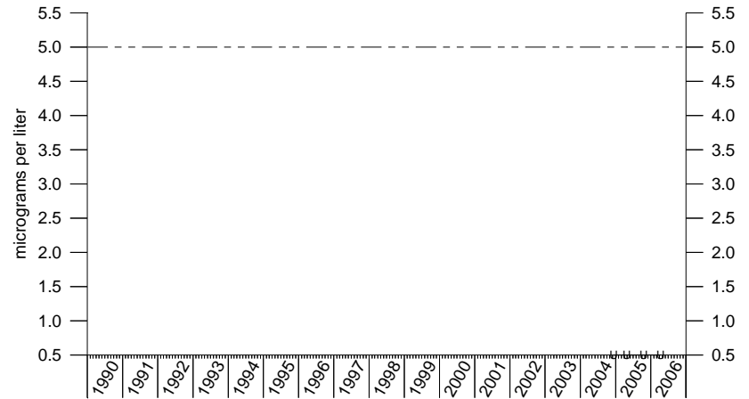
Tetrachloroethene IRA-22
