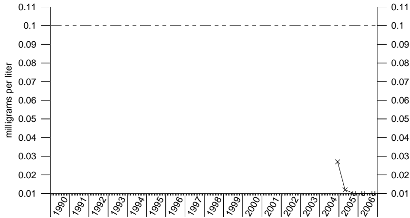
Chromium IRA-30
