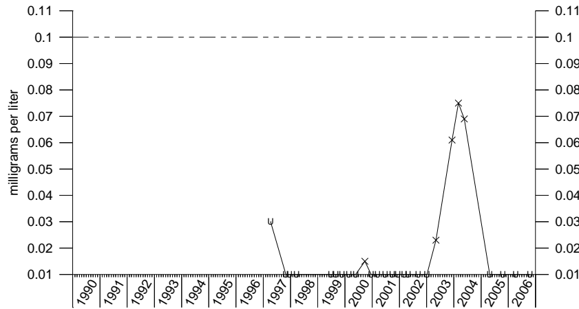
Chromium IRA-1
