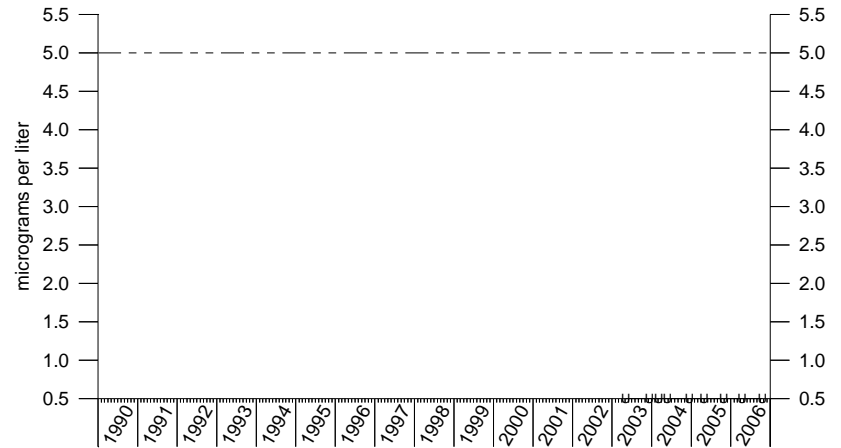
Tetrachloroethene IRA-14-4
