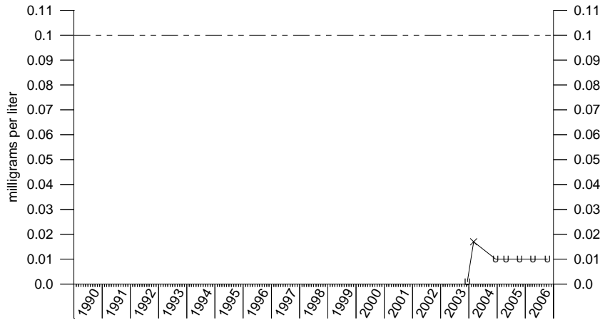
Chromium IRA-21
