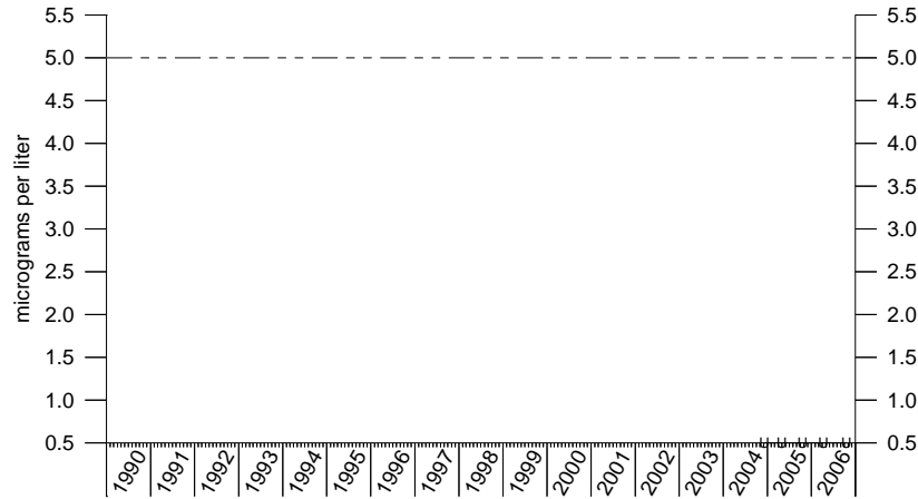
Tetrachloroethene IRA-30
