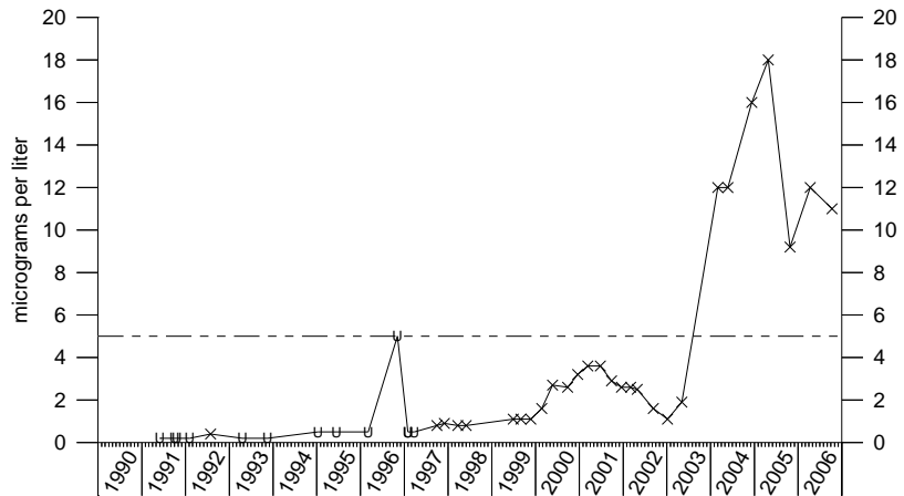
Tetrachloroethene IRA-5
