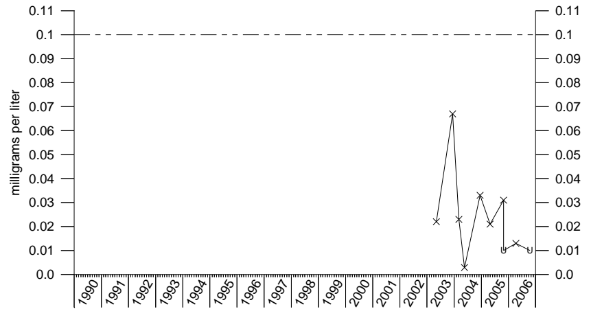
Chromium IRA-22
