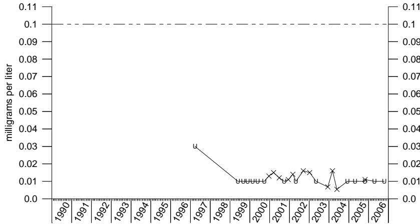
Chromium IRA-5
