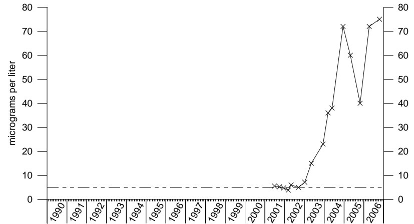
Trichloroethene IRA-13-210
