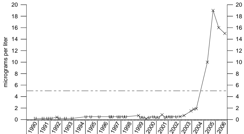
Tetrachloroethene IRA-1
