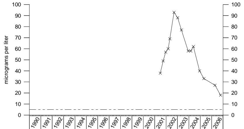
Trichloroethene IRA-13-210
