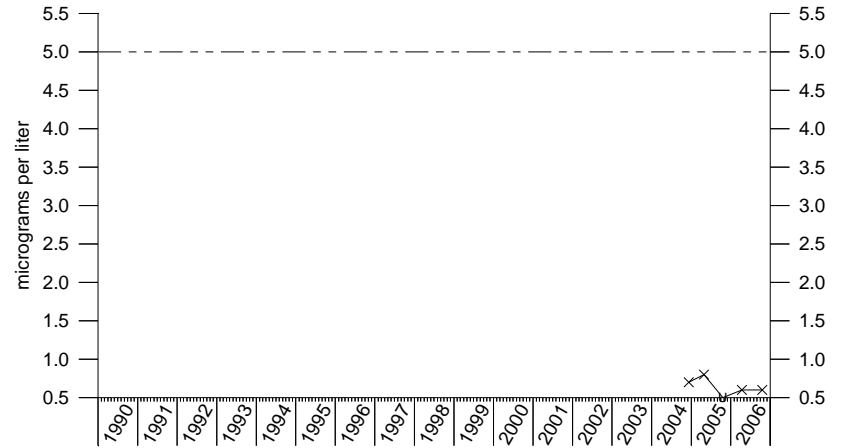
Tetrachloroethene IRA-29
