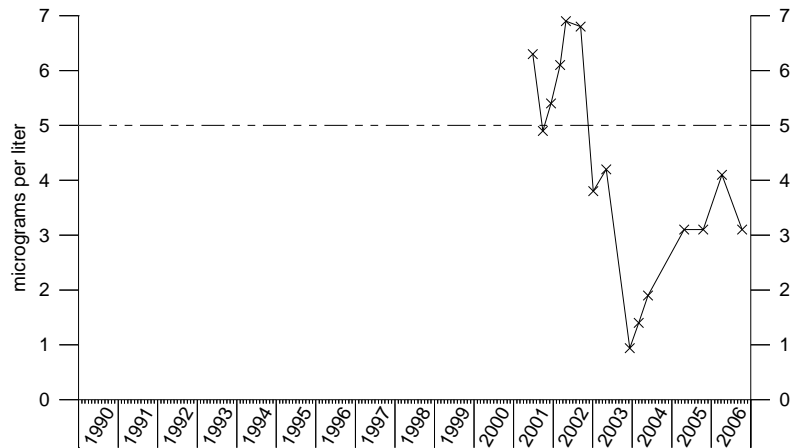
Trichloroethene IRA-12-210
