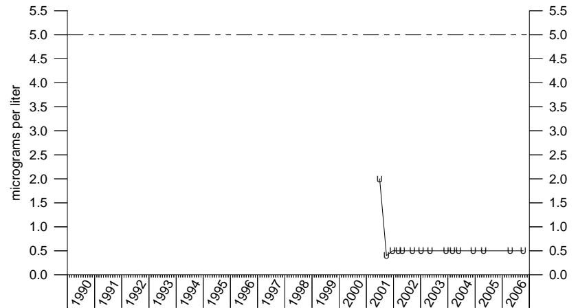
Tetrachloroethene IRA-13-210
