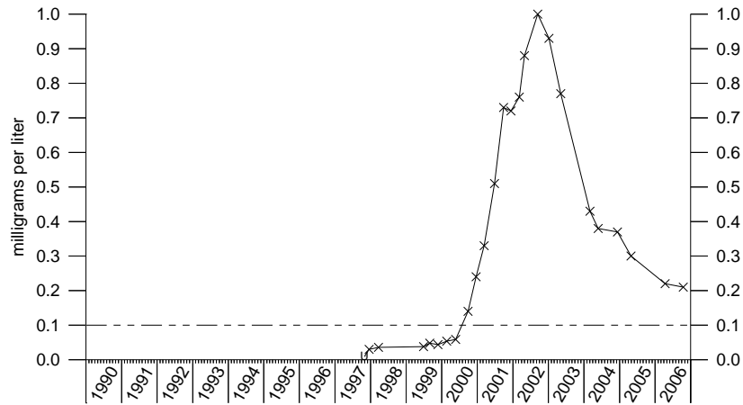
Chromium IRA-9
