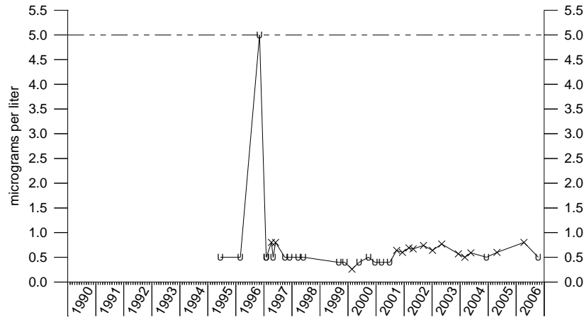
Tetrachloroethene IRA-9
