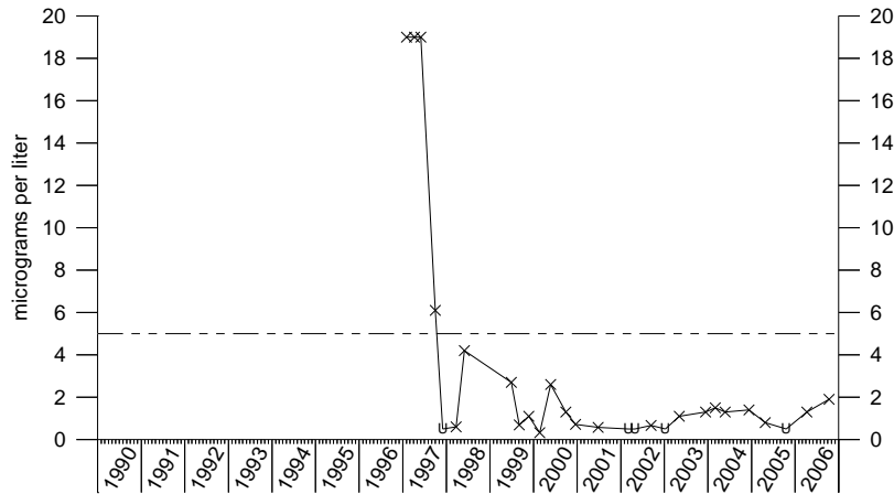
Trichloroethene IRA-12-210
