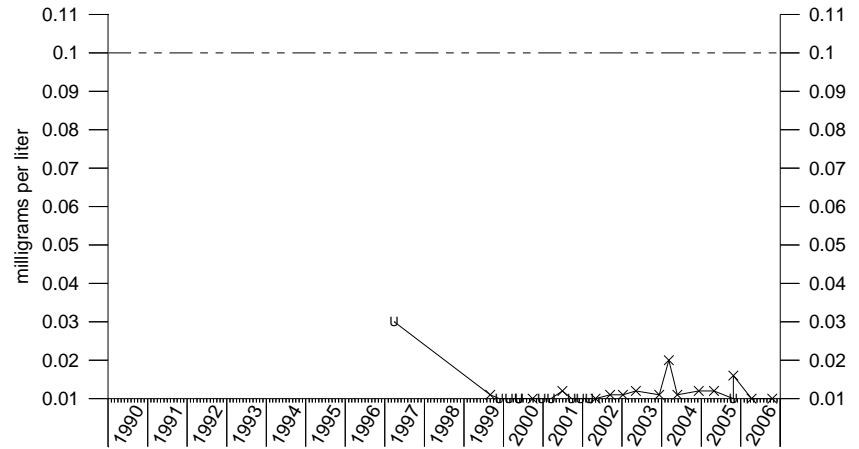
Chromium IRA-2
