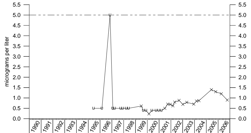
Tetrachloroethene IRA-6
