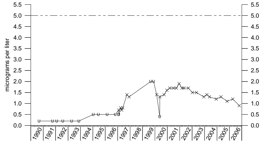
Tetrachloroethene IRA-2
