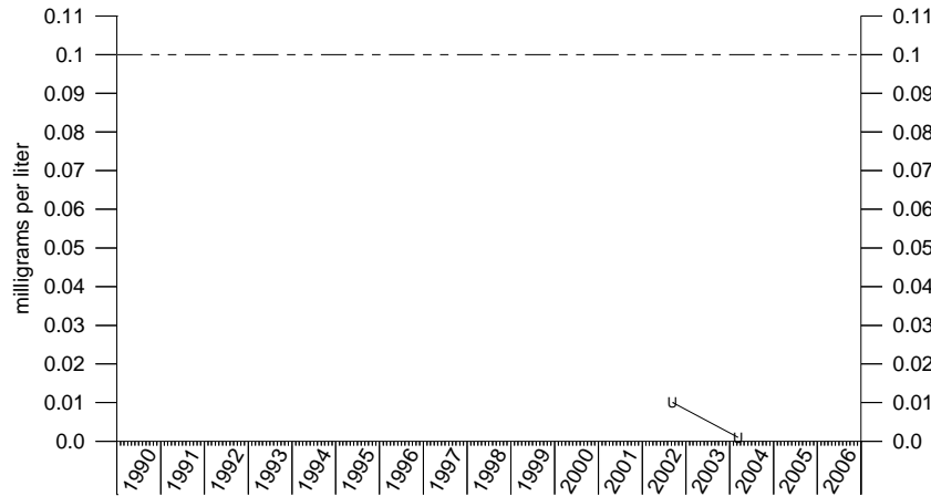
Chromium IRA-16
