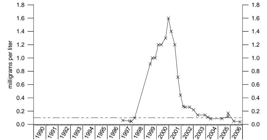
Chromium IRA-2
