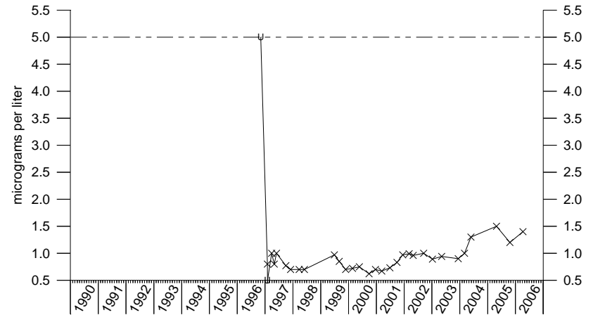
Tetrachloroethene IRA-8
