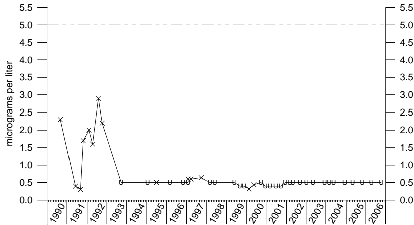
Tetrachloroethene IRA-1
