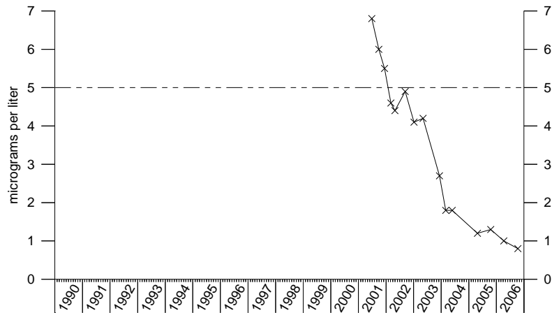
Tetrachloroethene IRA-12-210
