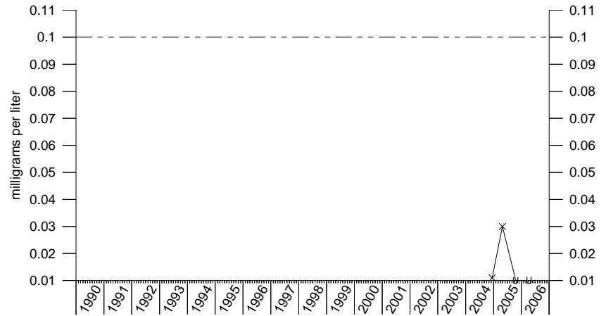
Chromium IRA-22
